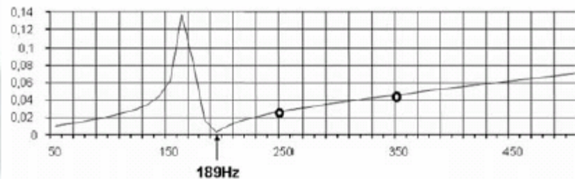
System busbar: impedance vs. frequency
